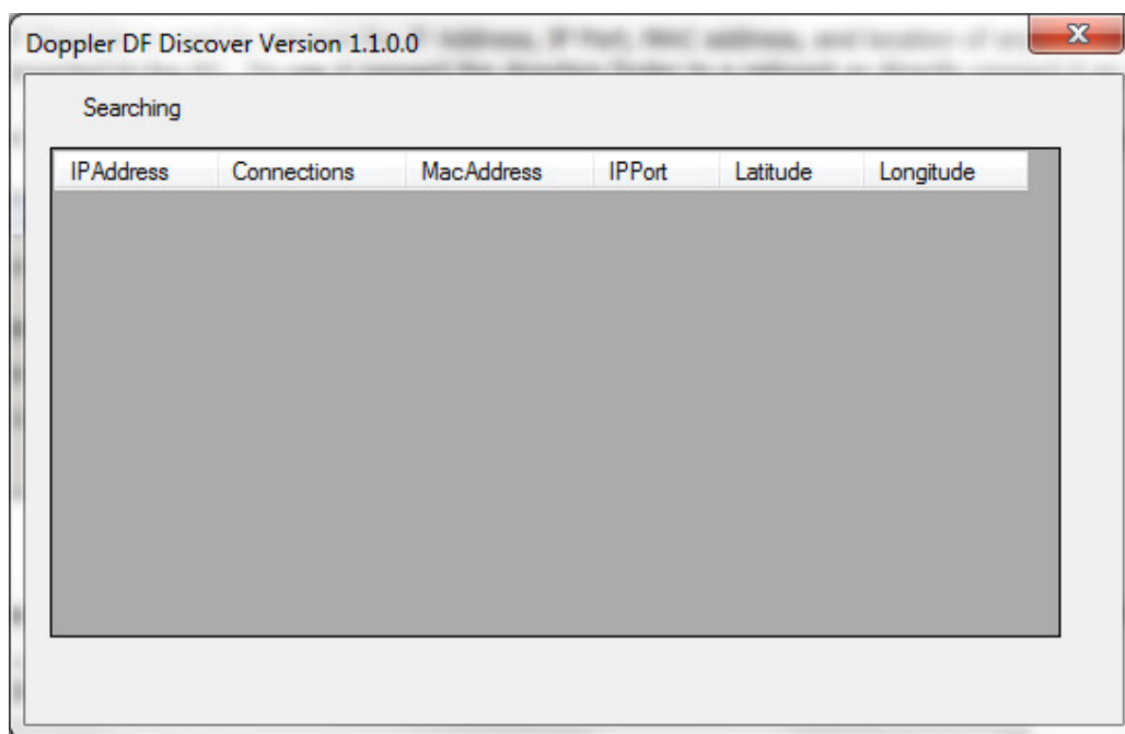
Figure 25: Initial Dialog
