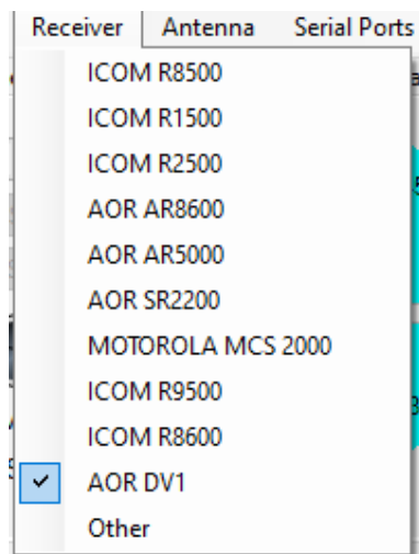
Figure 8: Receiver Menu
