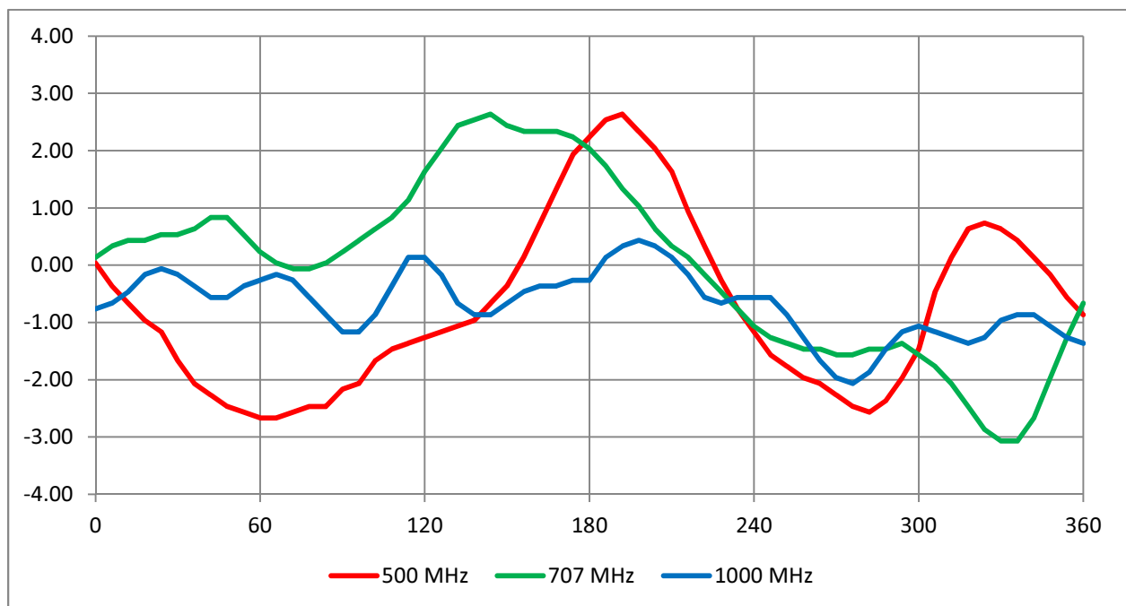
Figure 3 - Bearing Accuracy for DDF7093 (8THF) Antenna
